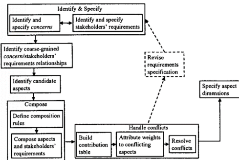
Fig. 9. AORE Model
